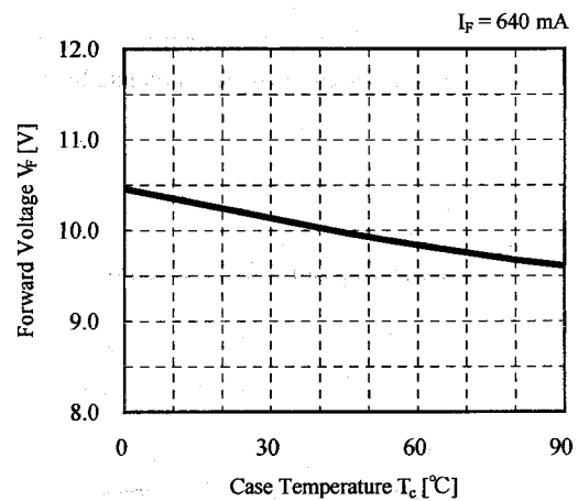
Case Temperature vs. Forward Voltage
