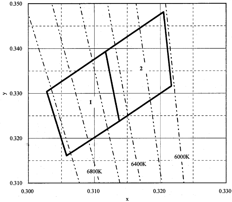
Chromaticity Diagram
