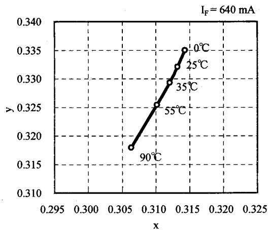
Chromaticity Coordinate vs. Case Temperature
