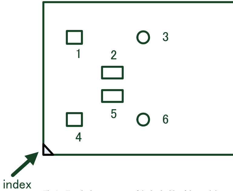
Fig.1 Terminal arrangement of the back side of the module
