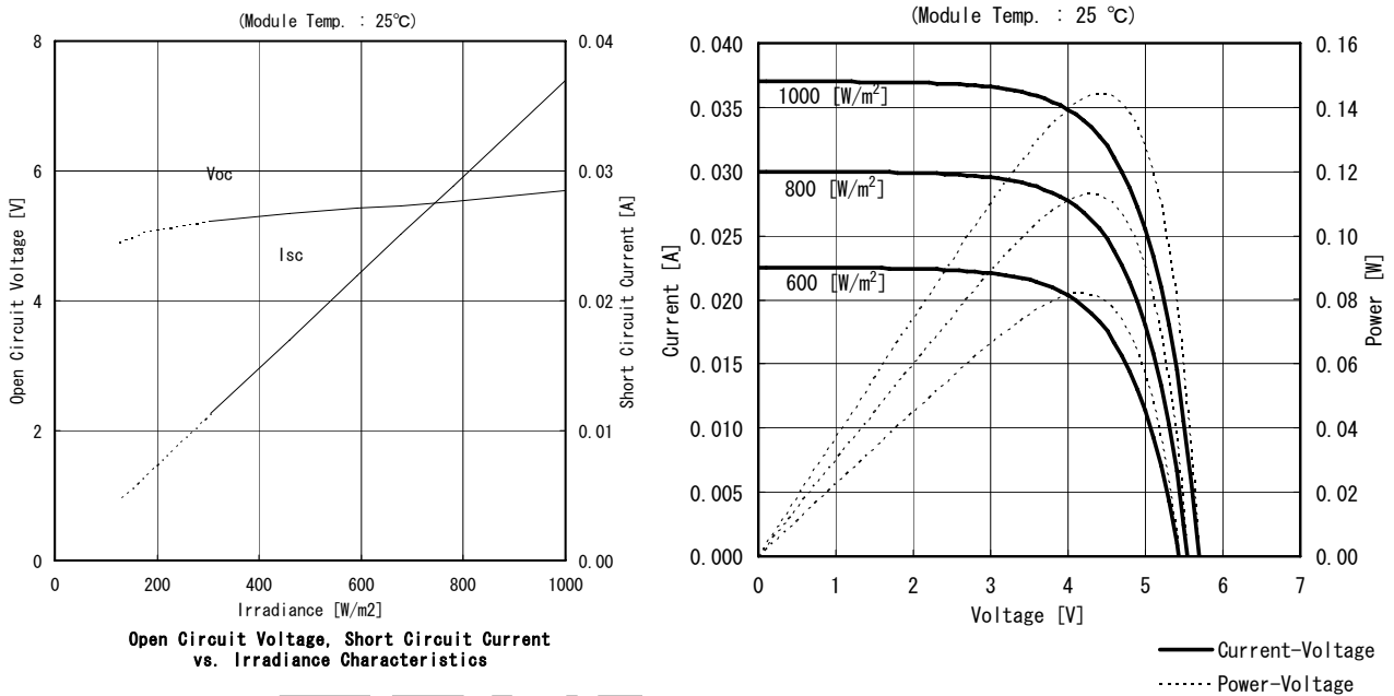
Current/Power vs. Voltage Characteristics
